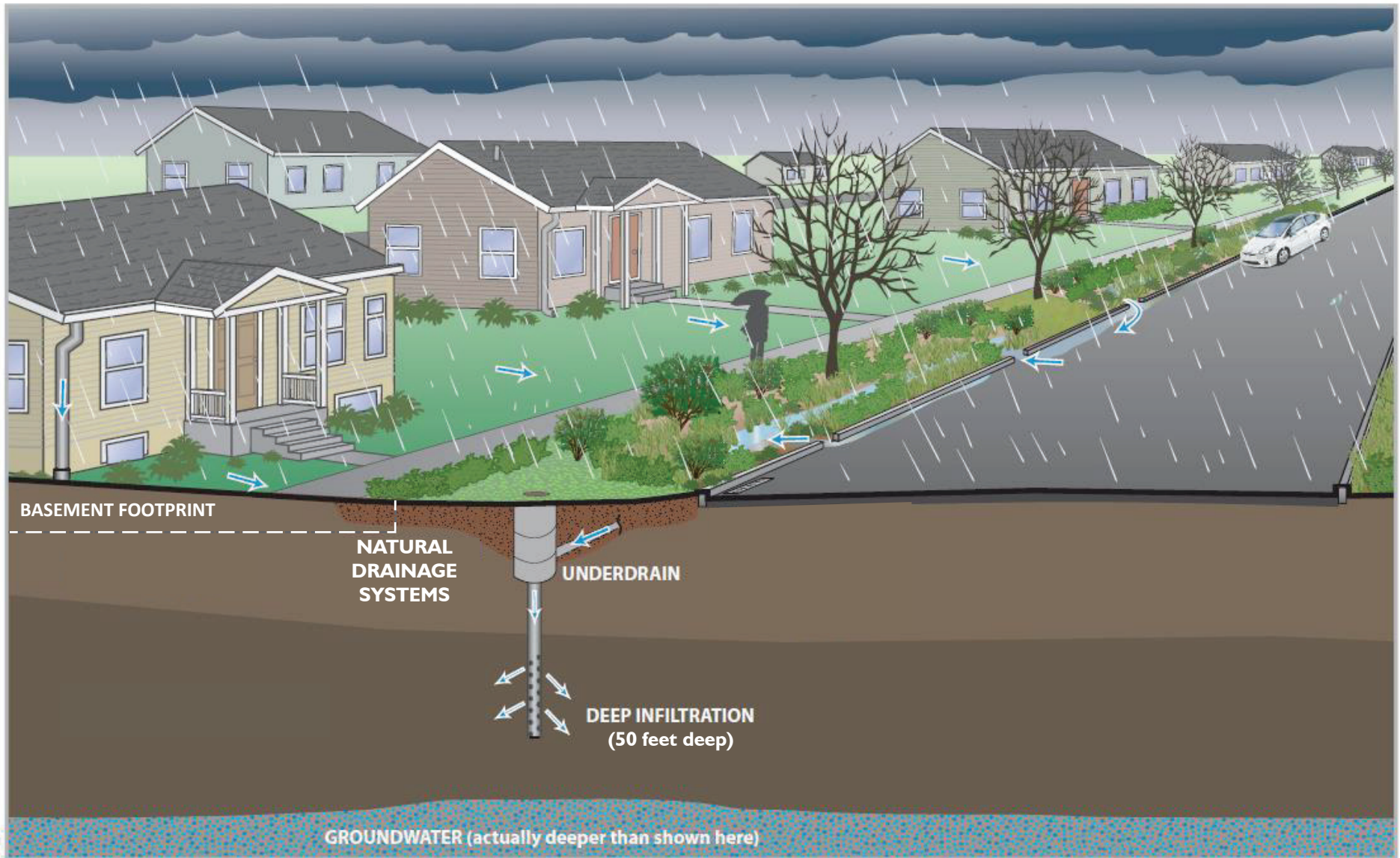
Example of natural drainage systems (NDS) installation and deep infiltration well Not to scale
